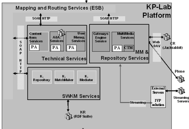
Figure 4: Architecture of the KP-Lab platform [9].
