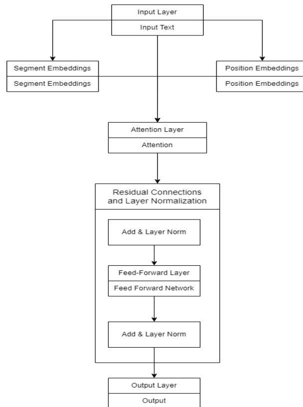
Figure 4: Proposed XLNet Architecture using fastText word embedding
