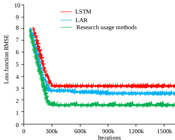
Figure 10: Comparison of loss functions among three algorithms Description: compares the change in loss function of the three algorithms during the iteration process
