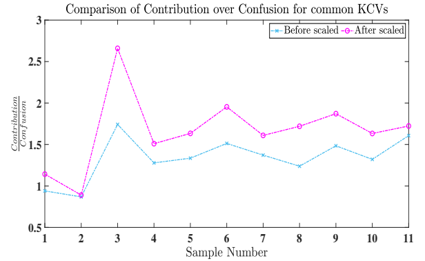
Figure 9: Confusion and contribution ratio for common KCVs from before and after mapping of data
