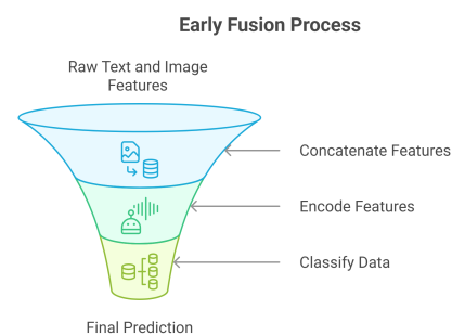
Figure 1: Early fusion pipeline
