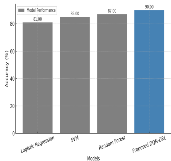
Figure 3: Accuracy comparison
