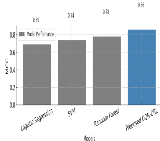
Figure 7: MCC comparison
