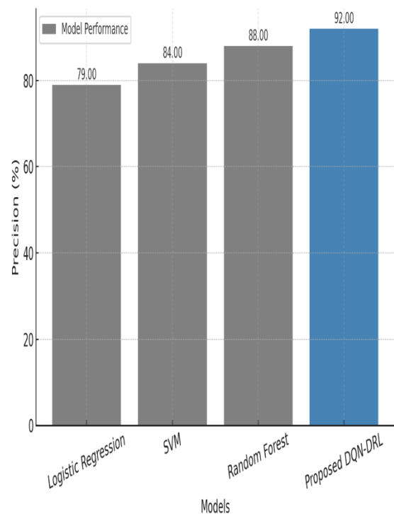
Figure 4: Precision comparison
