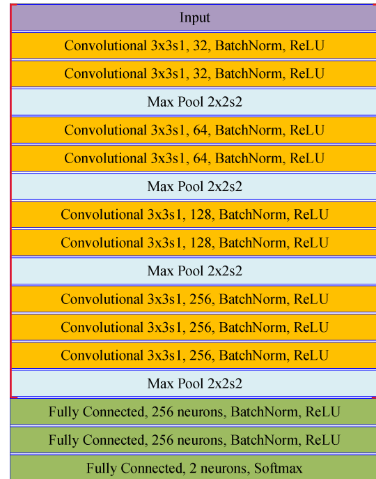
Figure 2: The CNN shared network in Multi-task BKNet is just the top part (marked by red lines) of the BKNet architecture [30], excluding the last three fully-connected layers.
