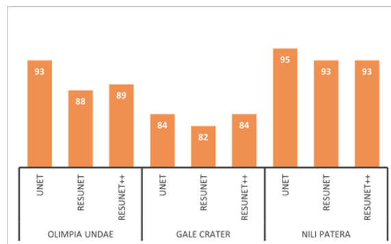
Figure 8: Accuracy assessment of results obtained from UNet, ResUNet and ResUNet++ models developed from CTX image in Olimpia Undae, Gale crater and Nili Patera region
